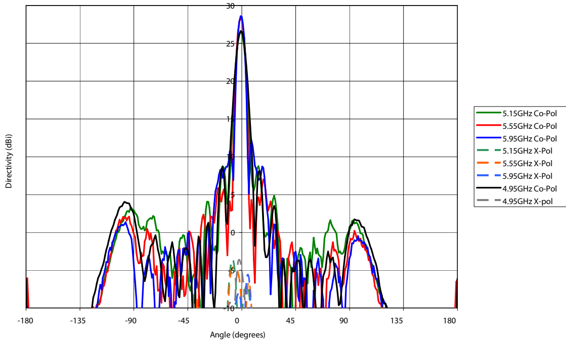
MPRD2449 Two-Foot Dual Polarized Reflector Antenna - H-Plane Radiation Patterns
