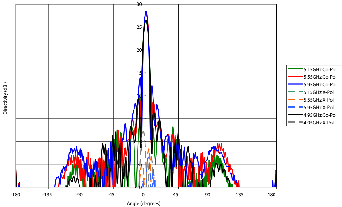
MPRD2449 Two Foot Dual-Polarized Reflector Antenna - E-Plane Radiation Patterns
