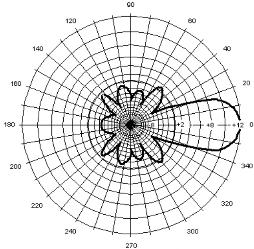
MYA45012 Horizontal Pattern
